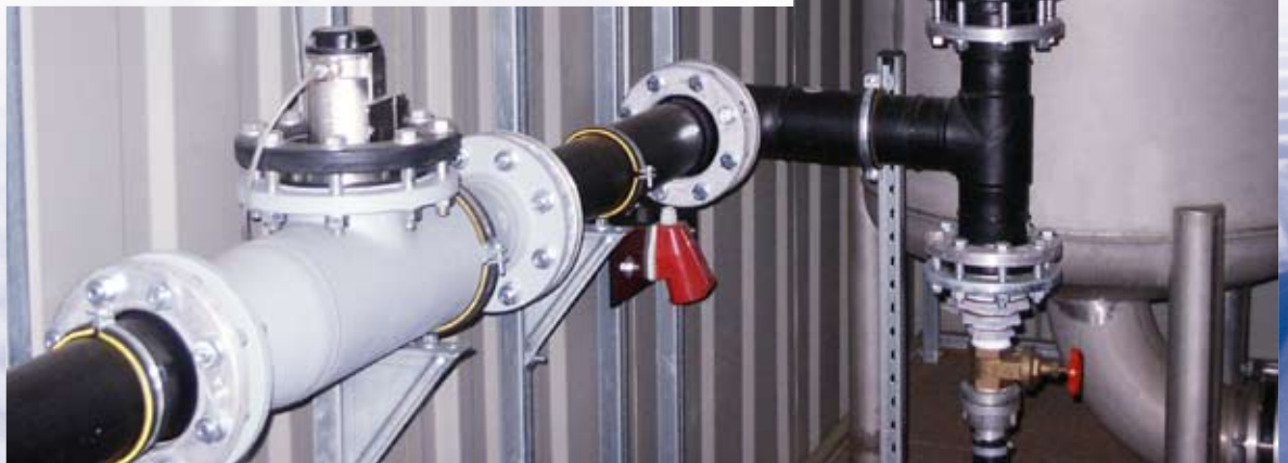
LEL detection system (inline) and liquid separator (detonation proof)
